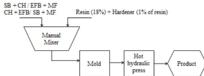
Fig. 3. Schematic of the process involved in the production of roof insulation fibreboard
