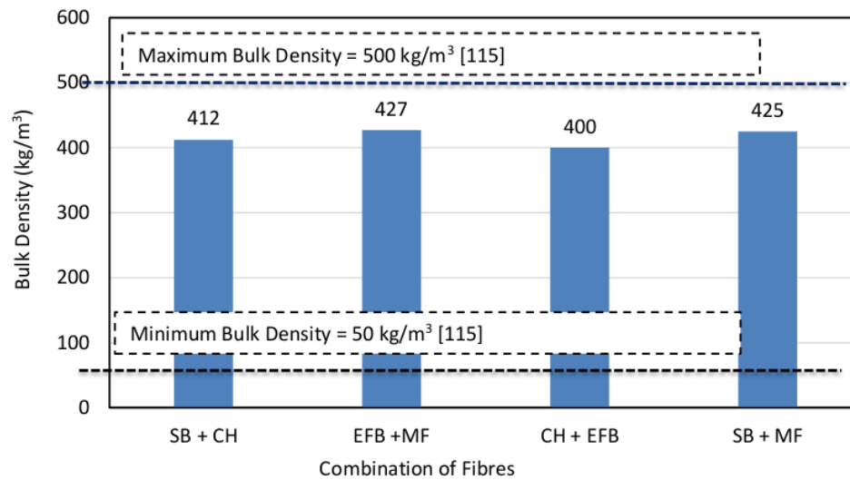
Fig. 6. Result bulk density test of different samples
