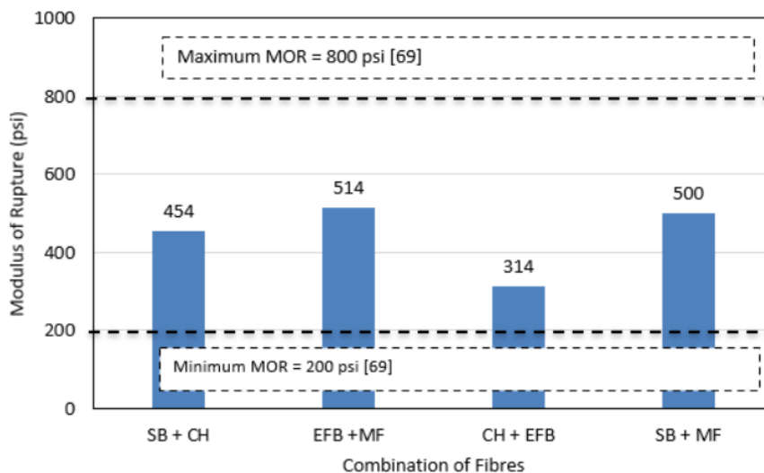
Fig. 8. Result MOR test of different samples
