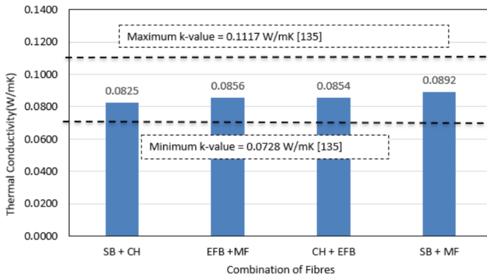
Fig. 9. Result of thermal conductivity value of different samples
