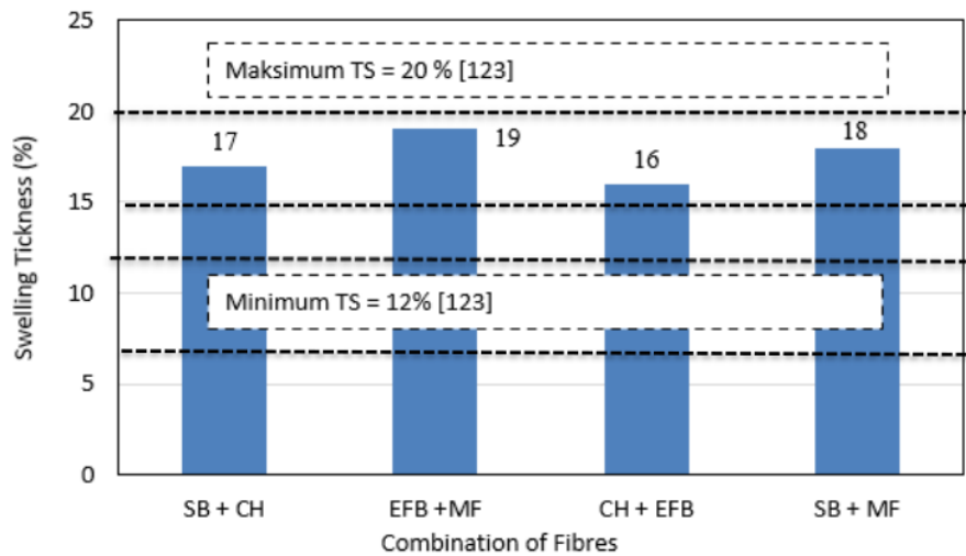
Fig. 7. Result swelling thickness of different samples
