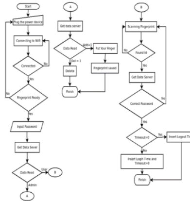
Gambar 2. Flowchart
