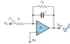
Fig. 5. Integrator circuit
