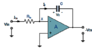
Fig. 4. Ideal integrator circuit
