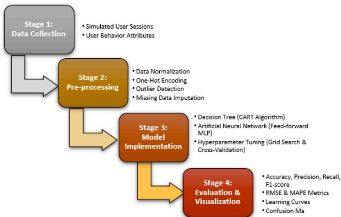
Figure 1: Research Methodology
