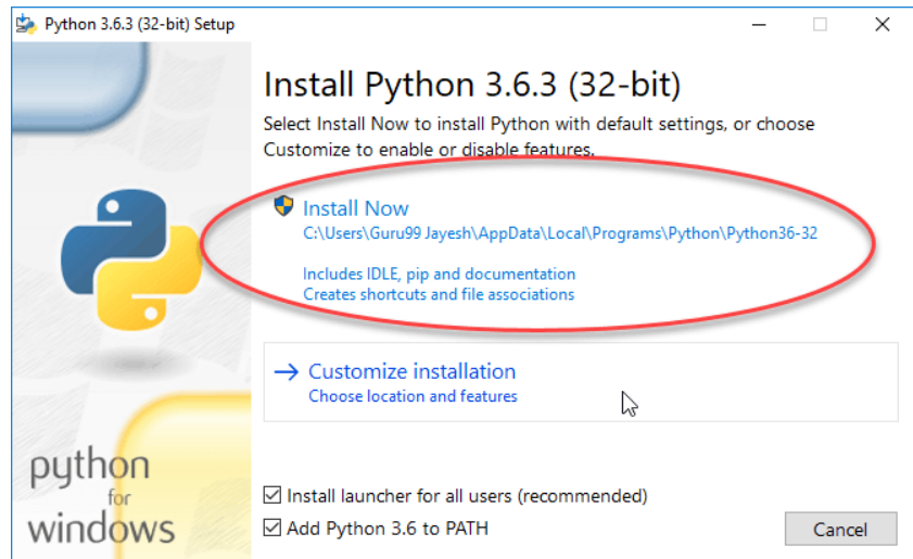
Gambar 1.7 Instalasi Python (2)
