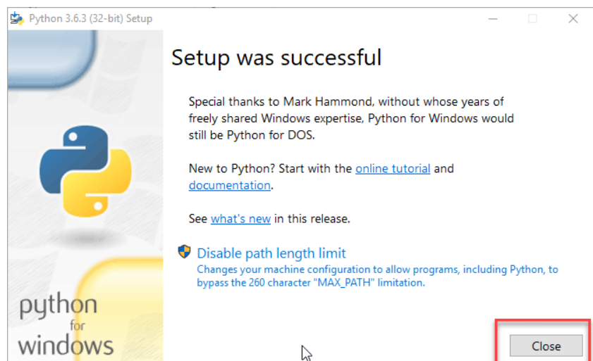
Gambar 1.8 Instalasi Python (3)
