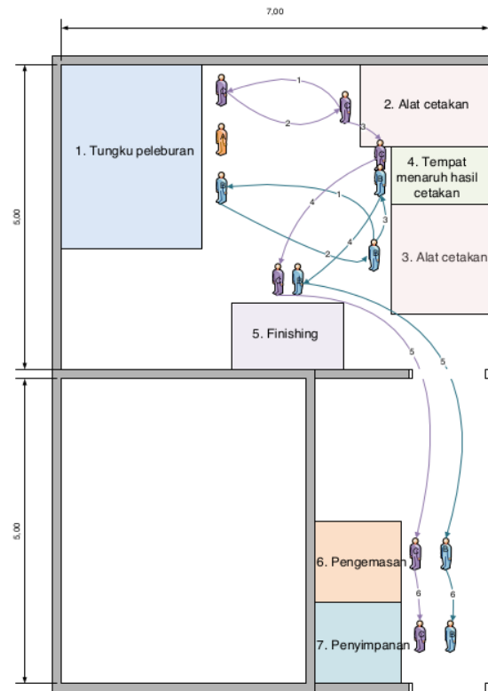
Gambar 5. Layout usulan
